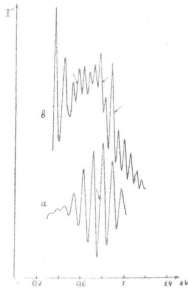
Fig. 1. a) I''(U) for films textured in direction [111] b) Interference I''(U) from film grains textured in directions [111] , [110] , [100] .
